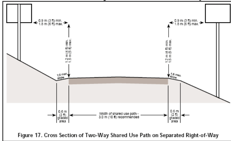
FIGURE 3.1 – Cross Section of Two-Way Shared Use Path on Separated Right-of-Way
