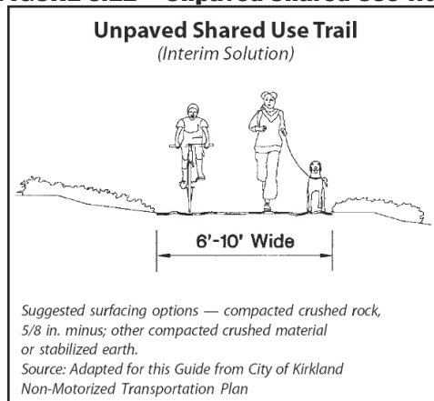
FIGURE 3.11 – Unpaved Shared Use Trail
